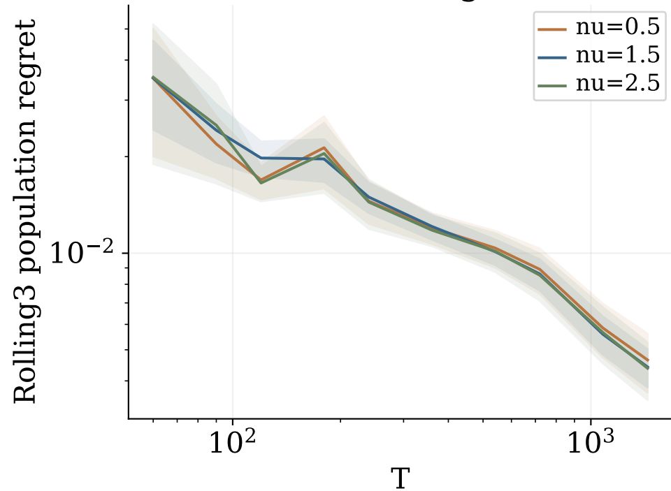
baseline original
